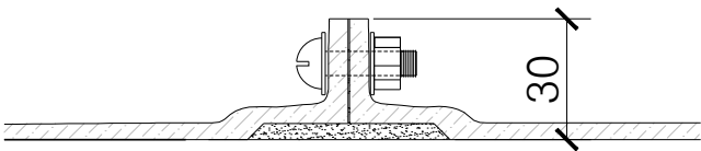
JOINT DETAIL
