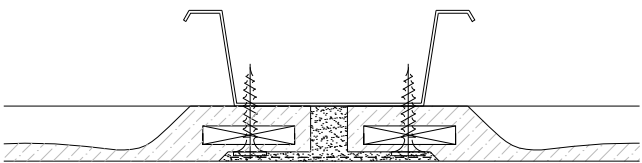
JOINT DETAIL
