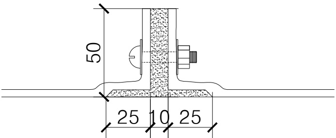
JOINT DETAIL
