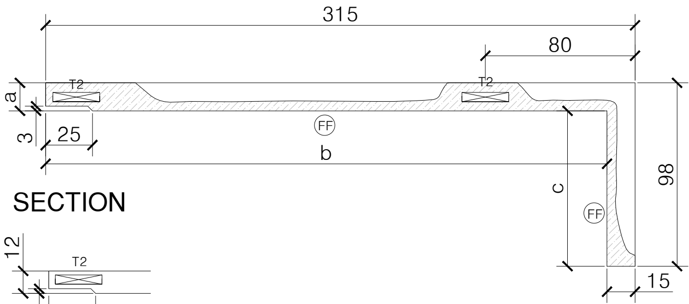
ALTERNATE DETAIL 1
