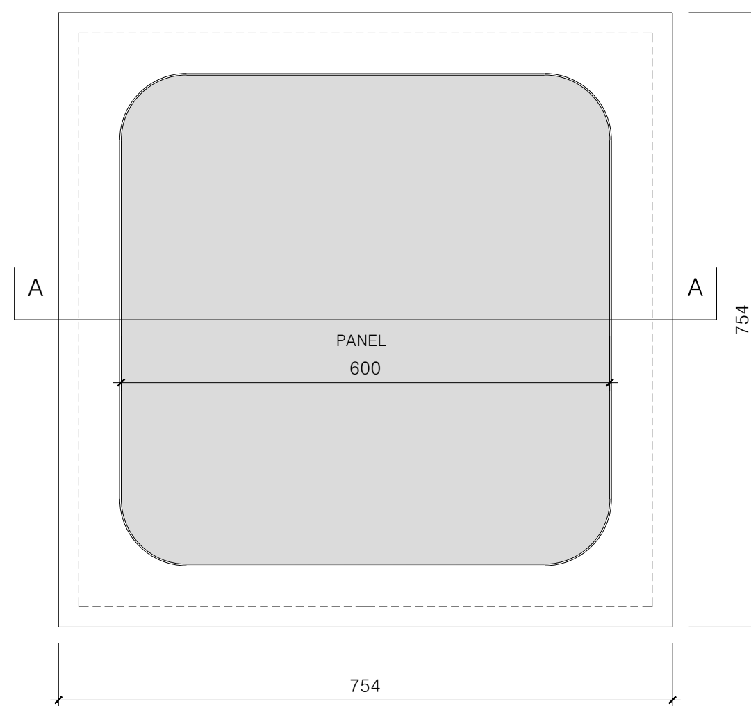
PANEL PLAN
